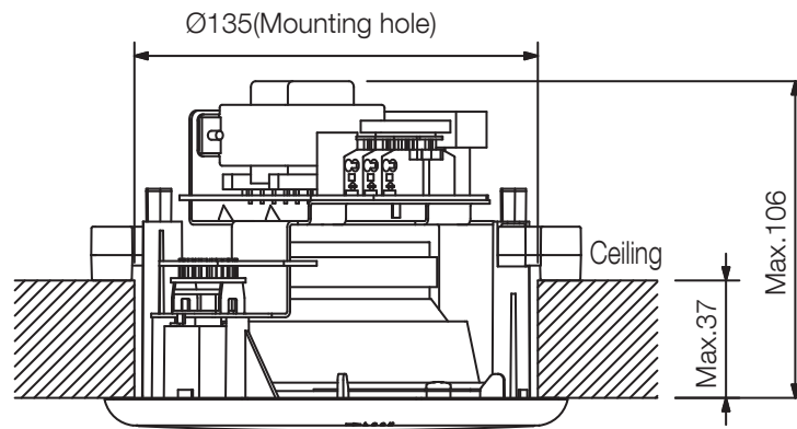
Ceiling mounting
